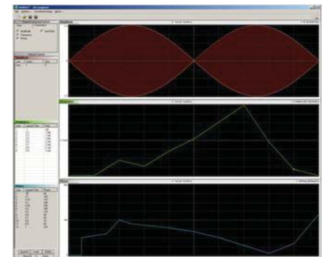
Figure 6: Combined AM, FM, and Phase Modulation in the 3D Composer
