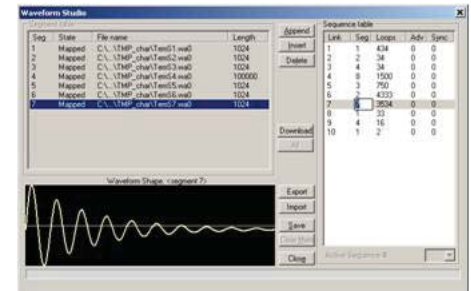
Figure 5: Sequence Definition in Waveform Studio
